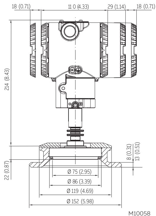
Figure 27 266GRT, 266ART with barrel housing and direct mount seal S26SS Sanitary flush (For dimensions of S26 seals refer to the S26 data sheet)
