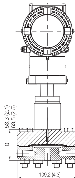
Figure 19 266GRT, 266ART with barrel housing and direct mount seal S26TT off-line threaded flange
