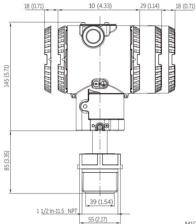
Figure 31 266GRT, 266ART with barrel housing and direct mount seal S26KN pulp and paper 1 1/2 in. NPT threaded connections
